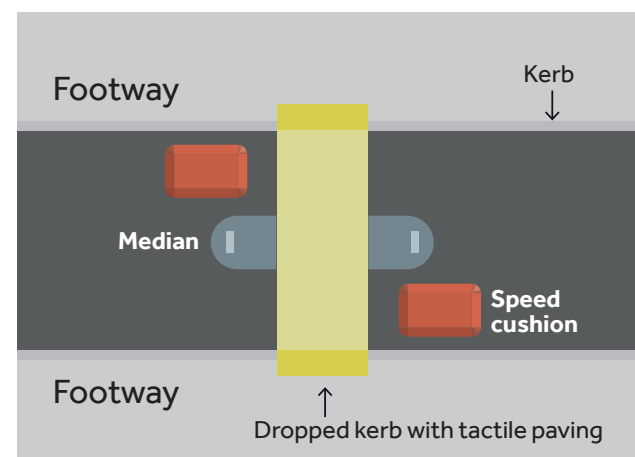
Figure 29: Speed cushion placement to benefit pedestrians crossing (not to scale)
